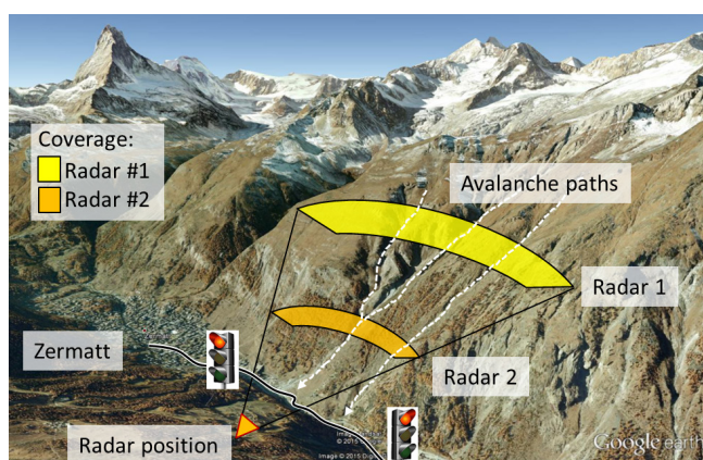
Figure 2: Overview of the alarm system in Zermatt. The radars are mounted on the opposite side of the valley.
