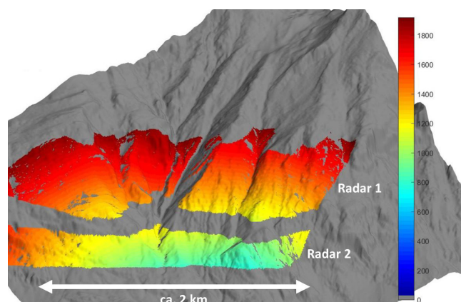
Figure 3: The radars monitor a total area of roughly two square km. The color in this graph indicates the distance to the radar in meters.
